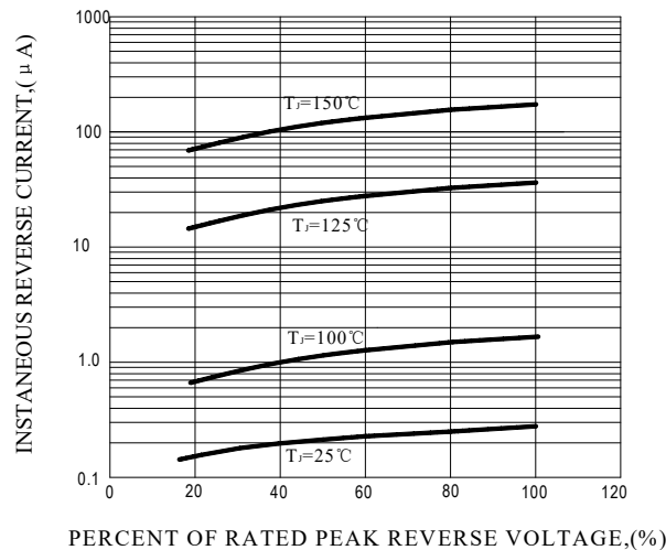
FIG.5-TYPICAL REVERSE CHARACTERISTICS
